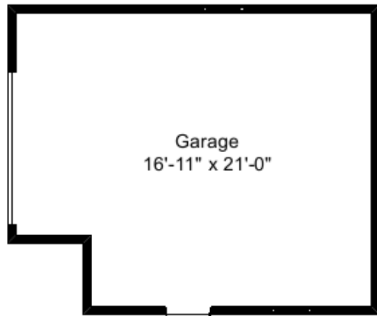
Garage Plan Ceiling Height = 8'-10"
