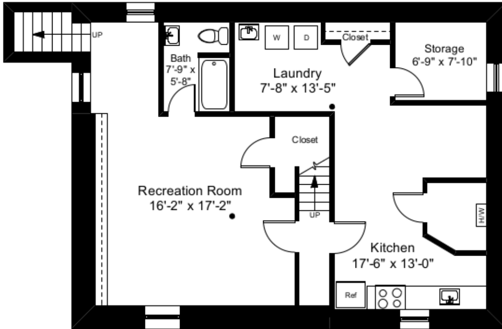
Lower Level Plan Ceiling Height = 6'-9"
