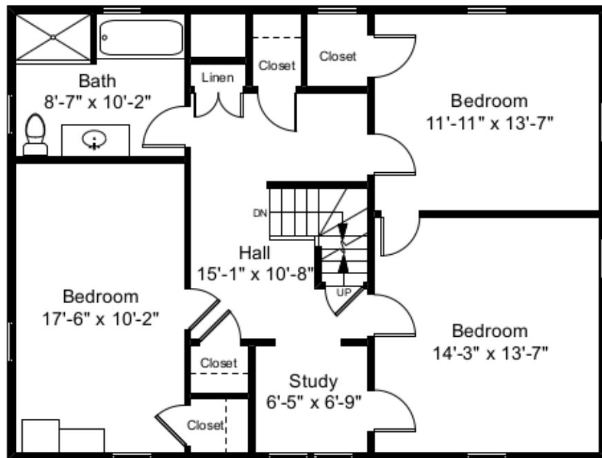
Second Floor Plan Ceiling Height = 8'-5"
